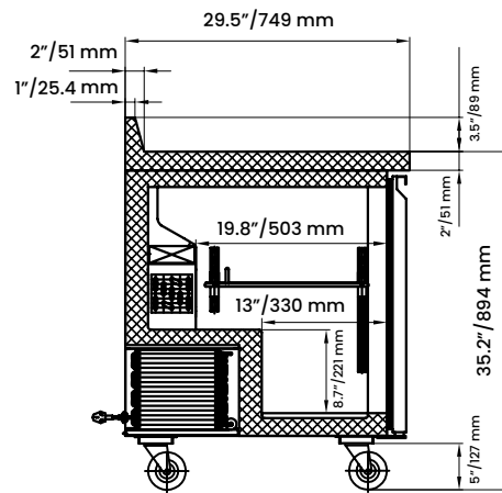
SECTION VIEW
