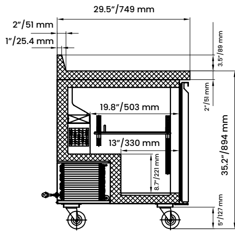
SECTION VIEW
